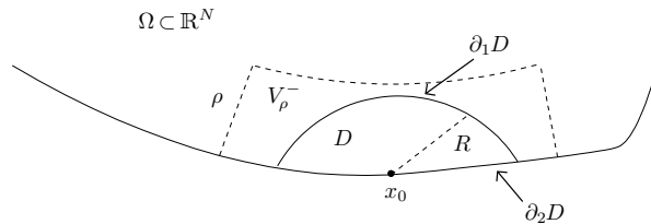
Fig. 1. The setting in the proof of Theorem 2.1
